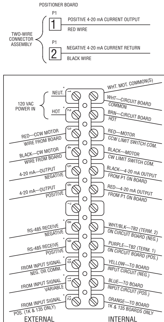
Figure 2 – Wiring of DFP17 120 VAC Digital Positioner with 4-20 mA position output
