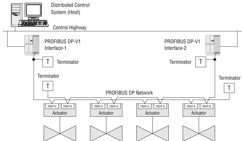
Figure 13.4b – Typical PROFIBUS DP Network with Redundancy Option (Dual Master)
