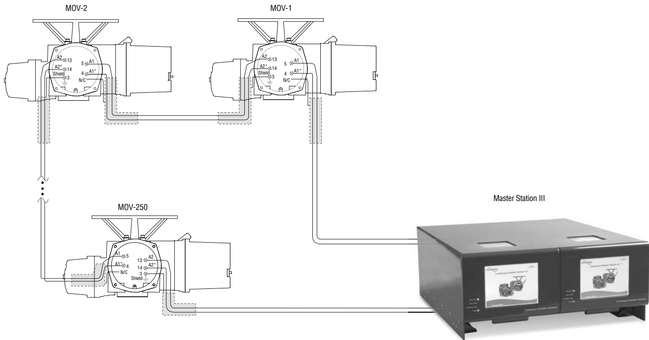
Figure 13.1 – Typical Modbus Network Wiring Diagrams – Redundant Bi-Directional Loop
