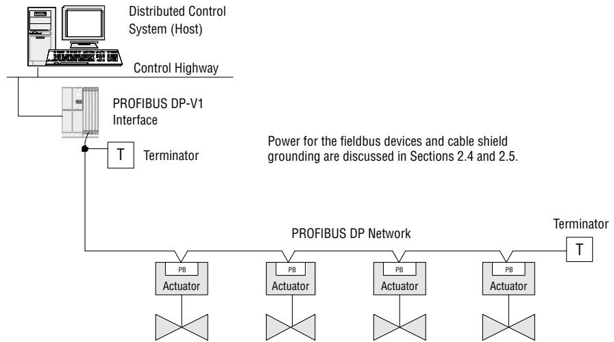
Figure 13.4 – Typical PROFIBUS DP Network (Daisy Chain Shown)
