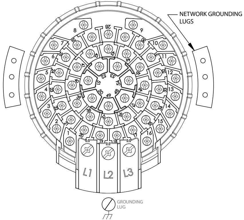
Figure – 11.1 MX/QX terminal block
