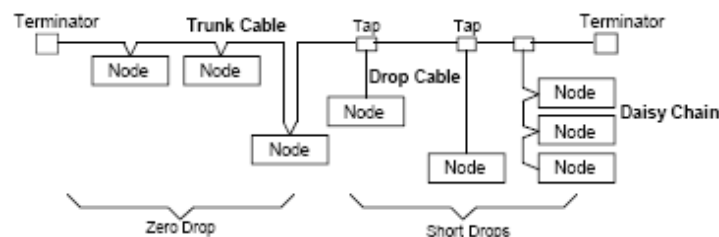
Figure 13.5 – Typical DeviceNet Network
