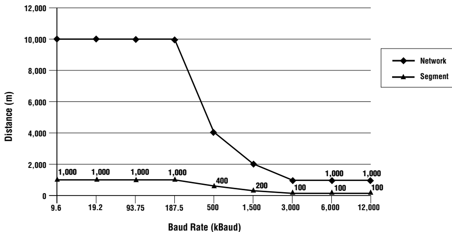
Figure 13.3 – PROFIBUS Distance vs. Baud Rate Chart
