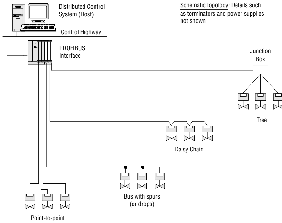
Figure 13.4c – Typical PROFIBUS PA Network
