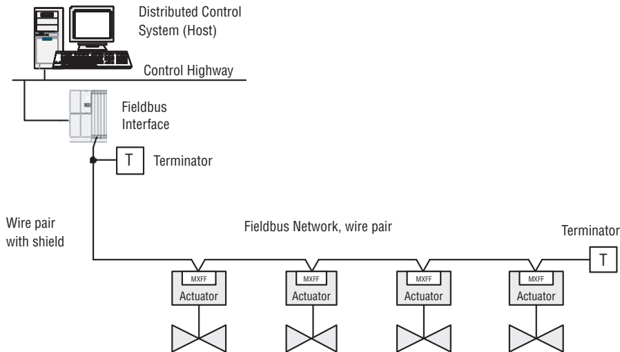
Figure 13.2 – Typical Foundation Fieldbus Network with DCS or PLC as the Host System
