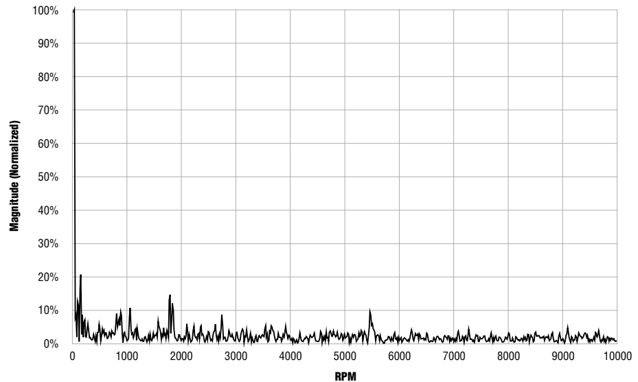
Figure 8.1 – FFT of a sound, efficient worm gear set
