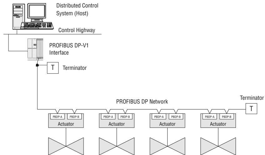
Figure 13.4a – Typical PROFIBUS DP Network with Redundancy Option (Single Master)
