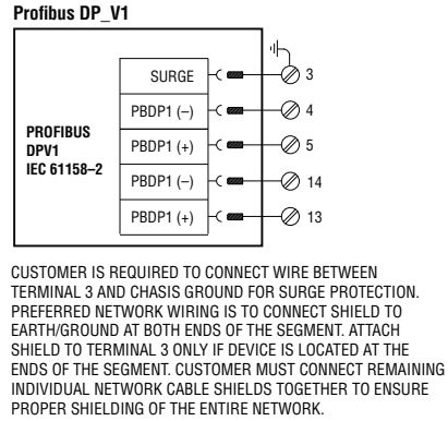
Figure 12.3 – DDC, FOUNDATION Fieldbus, Profibus DP_V1, Redundant Profibus DP_V1, and Profibus PA, and DeviceNet Network Wiring Diagrams
