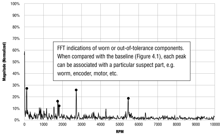
Figure 8.2 – FFT of an actuator exhibiting a specific component that is out of tolerance due to excessive wear.
